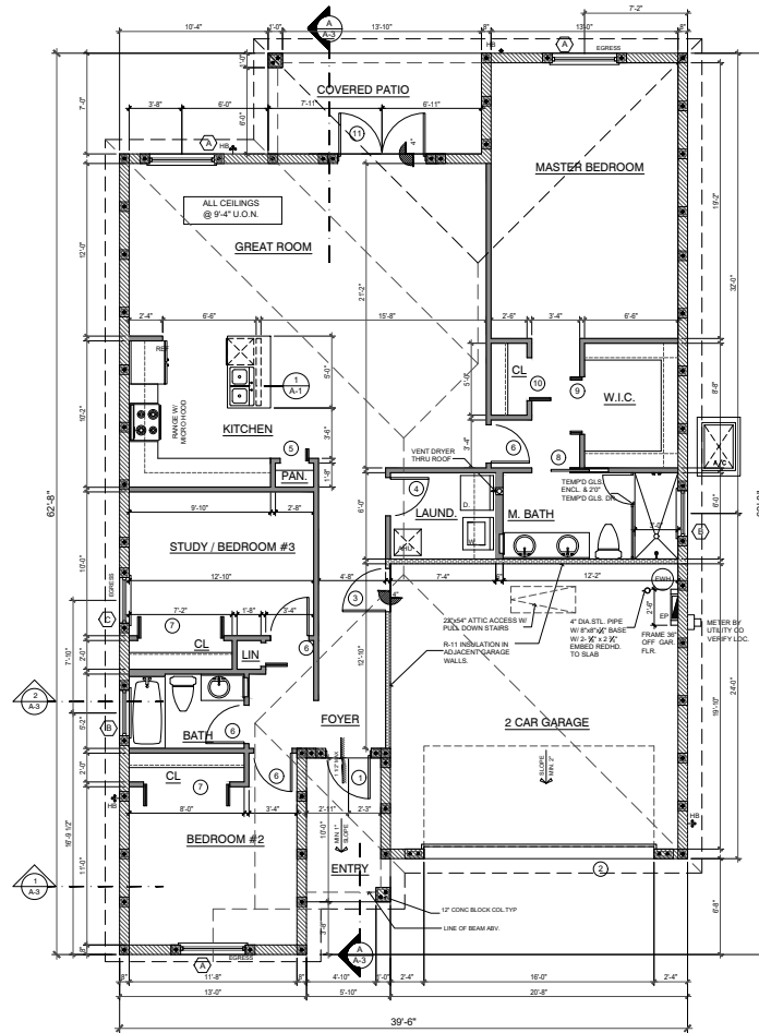
FLOOR PLAN
