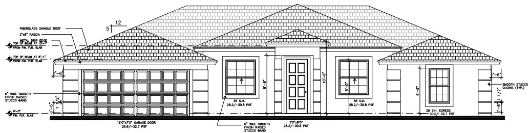
FRONT ELEVATION
